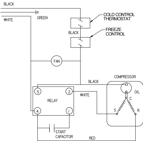
115V Wiring Diagram
