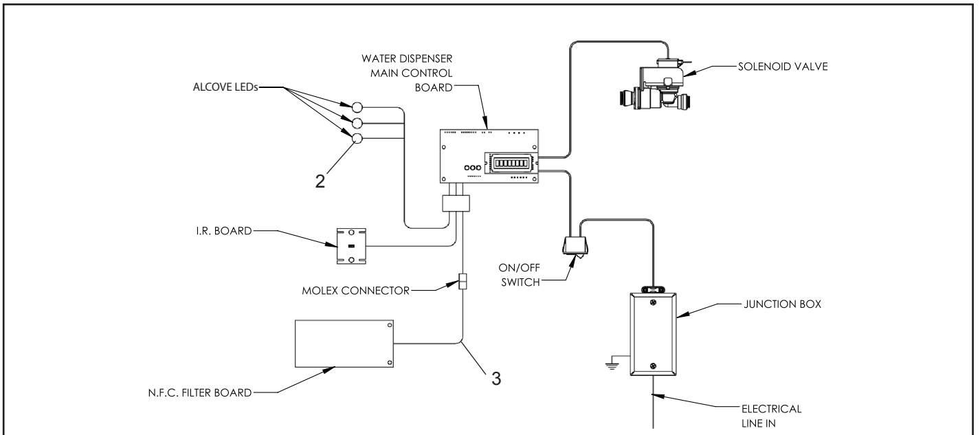
Electrical Diagram
