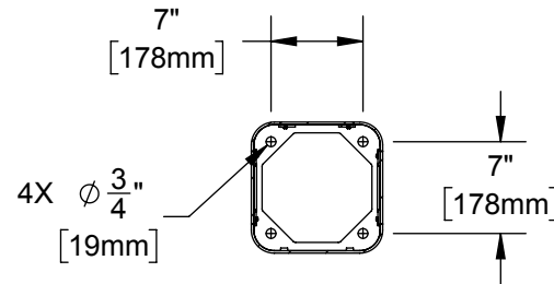
SECTION A-A INTERNAL PEDESTAL MOUNTING DETAIL
