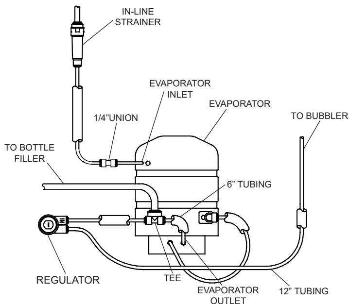
EMABF(WS) PLUMBING
