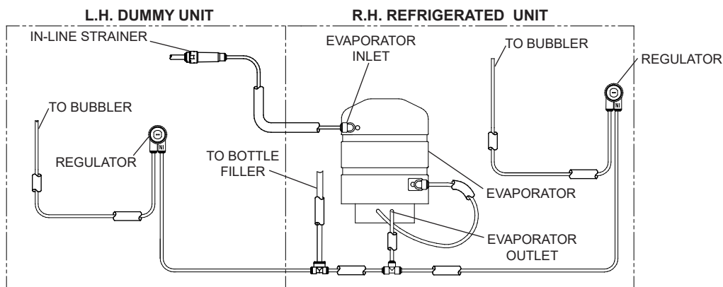
EMABF(WS) TWO LEVEL PLUMBING BOTTLE FILLER ON RH SIDE (SEE NOTE 2)
