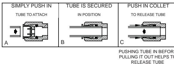
Figure 9 - Quick Connect Fittings
