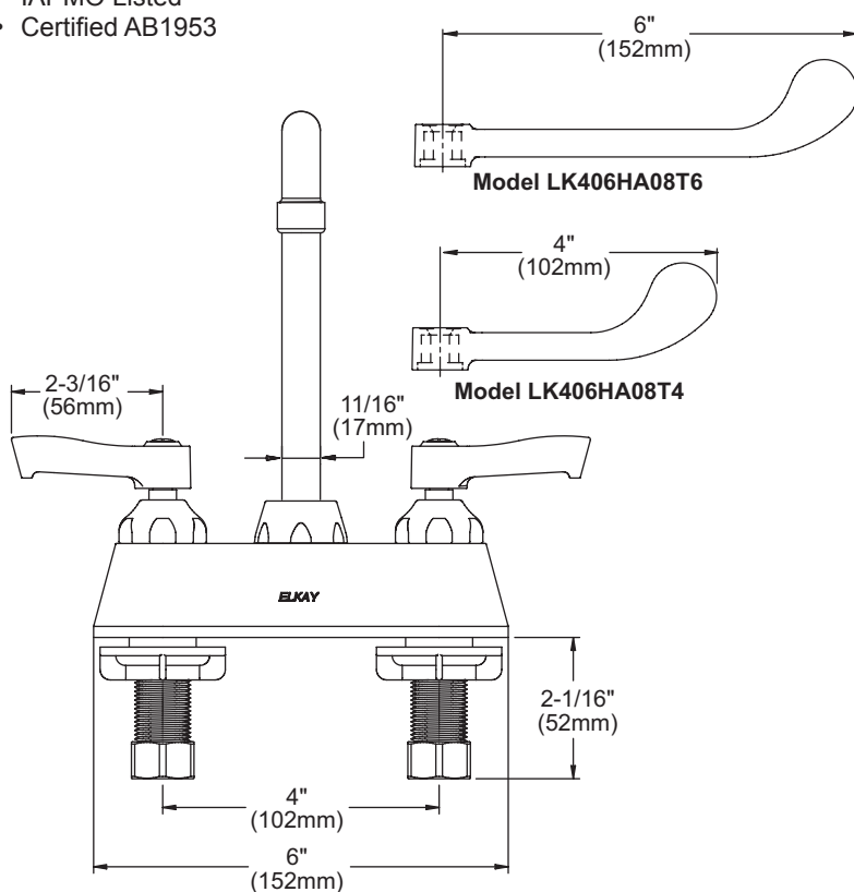
Model LK406HA08L2 FRONT VIEW
