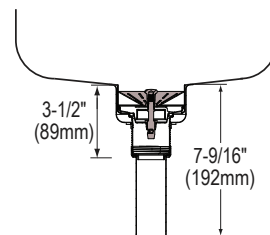
Sink with Drain Kit Installed
