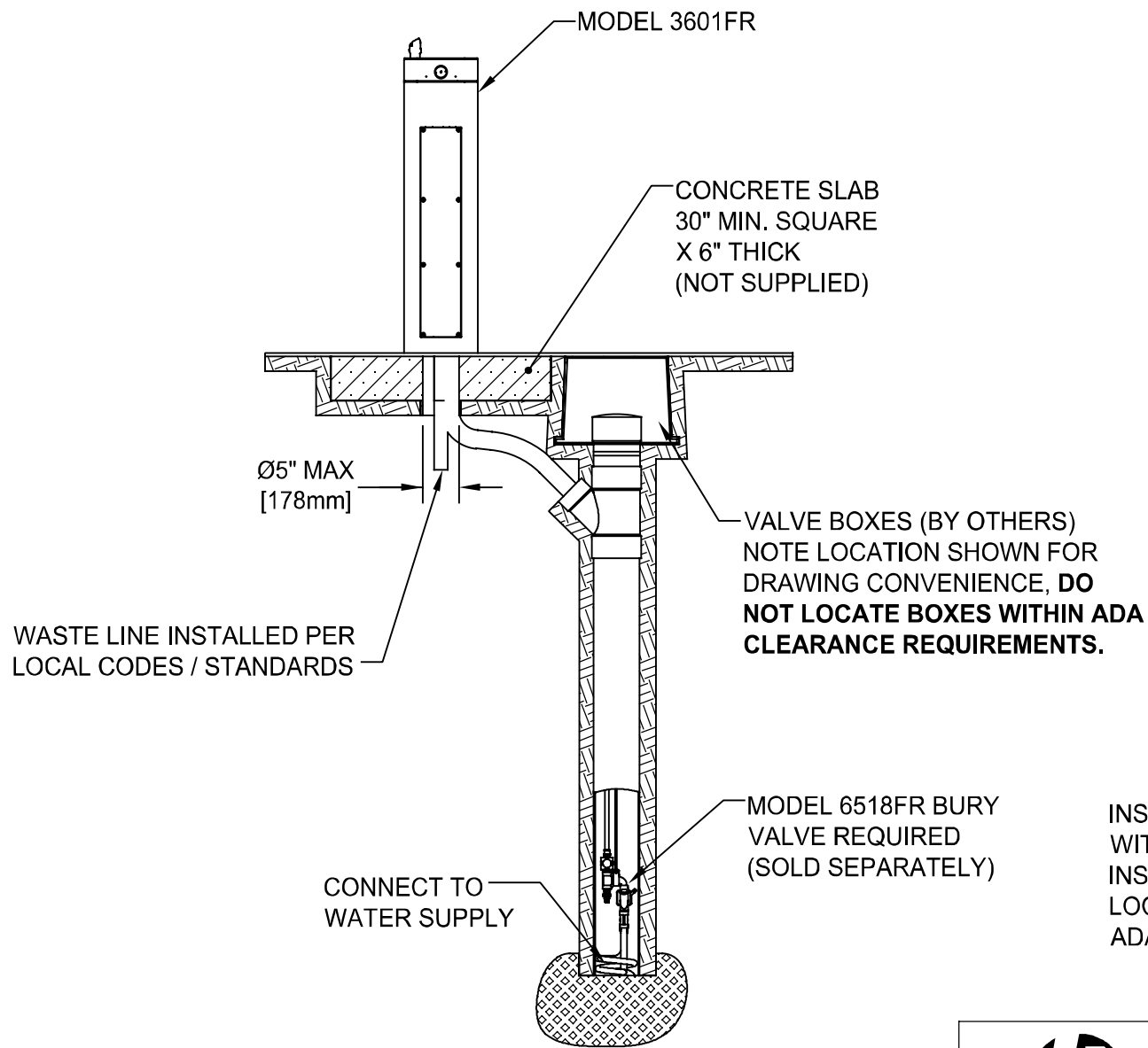
3601FR GENERAL BURY VALVE LAYOUT (FOR REFERENCE ONLY)
