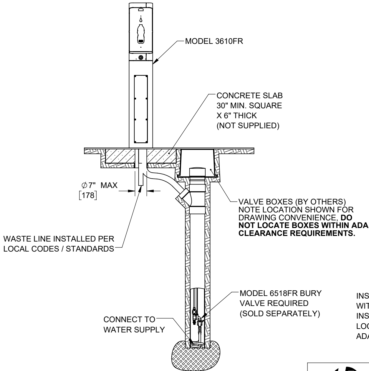
3610FR GENERAL BURY VALVE LAYOUT (FOR REFERENCE ONLY)
