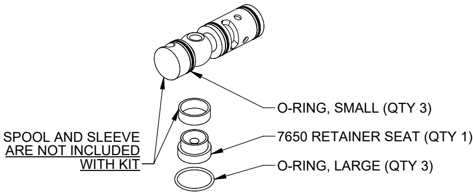
4 VRK7650 REPAIR KIT
