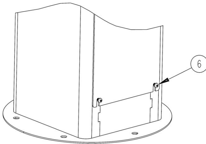
Fig.6 – Lower back panel positioning screws
