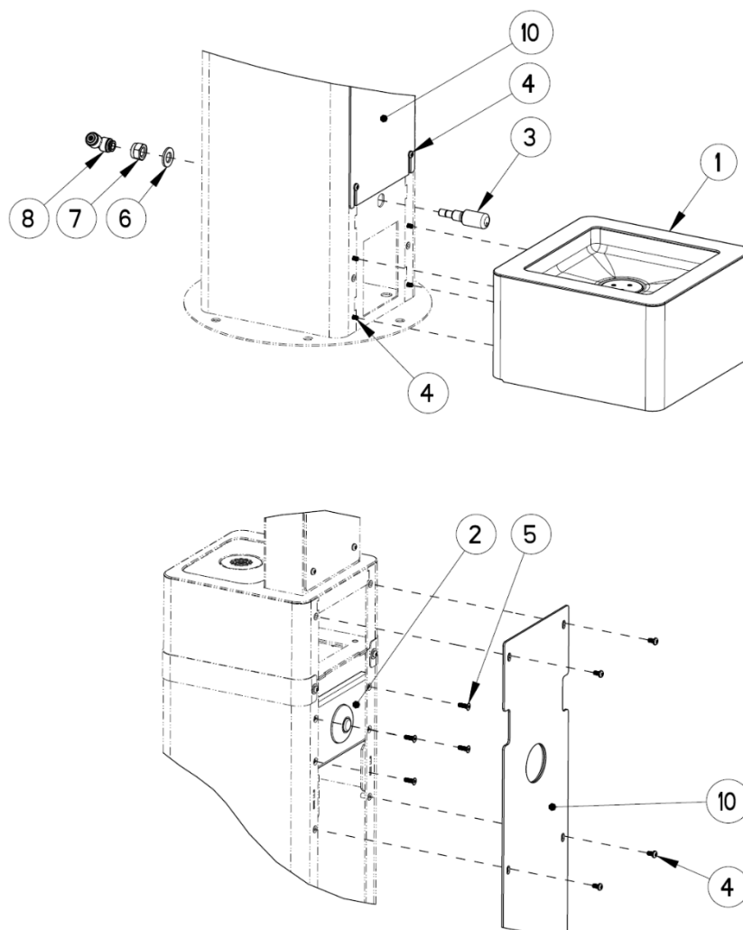
Fig. 12 - Pet bowl assembly
