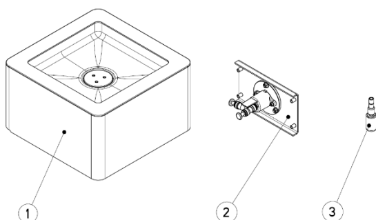
Fig. 10 - Pet bowl components
