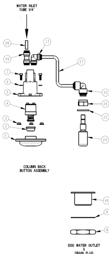
Fig. 13 – Pet bowl water circuit
