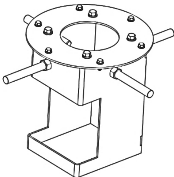
Fig.2 – Optional anchor assembly & filter access guideline
