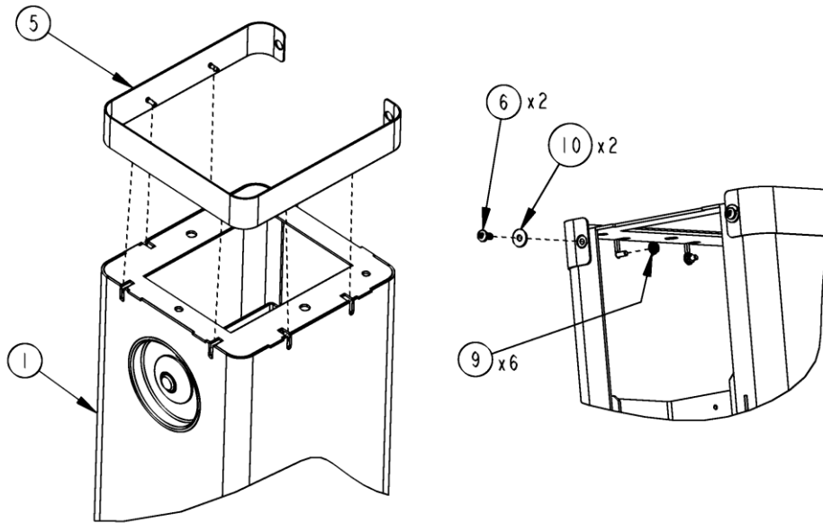
Fig. 3 – Aesthetic ring assembly
