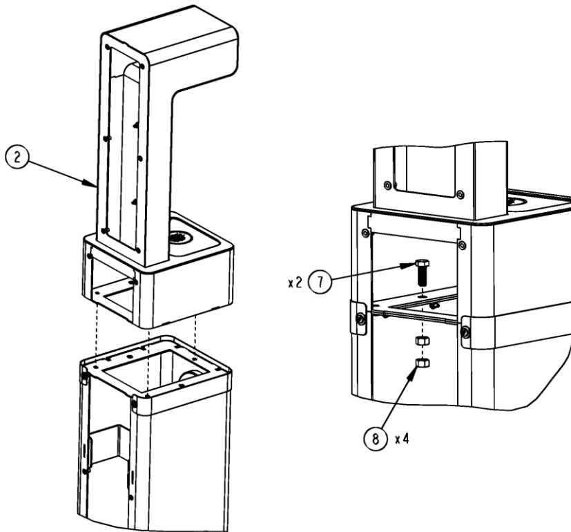
Fig.4 – Alcove assembly
