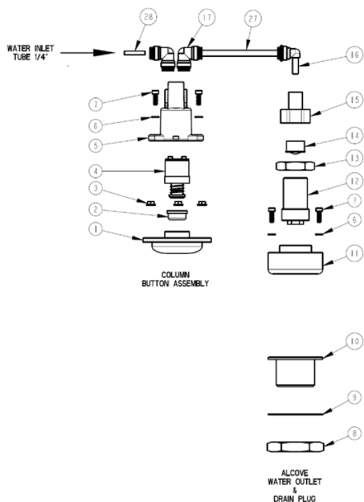
Fig. 9 – Water circuit
