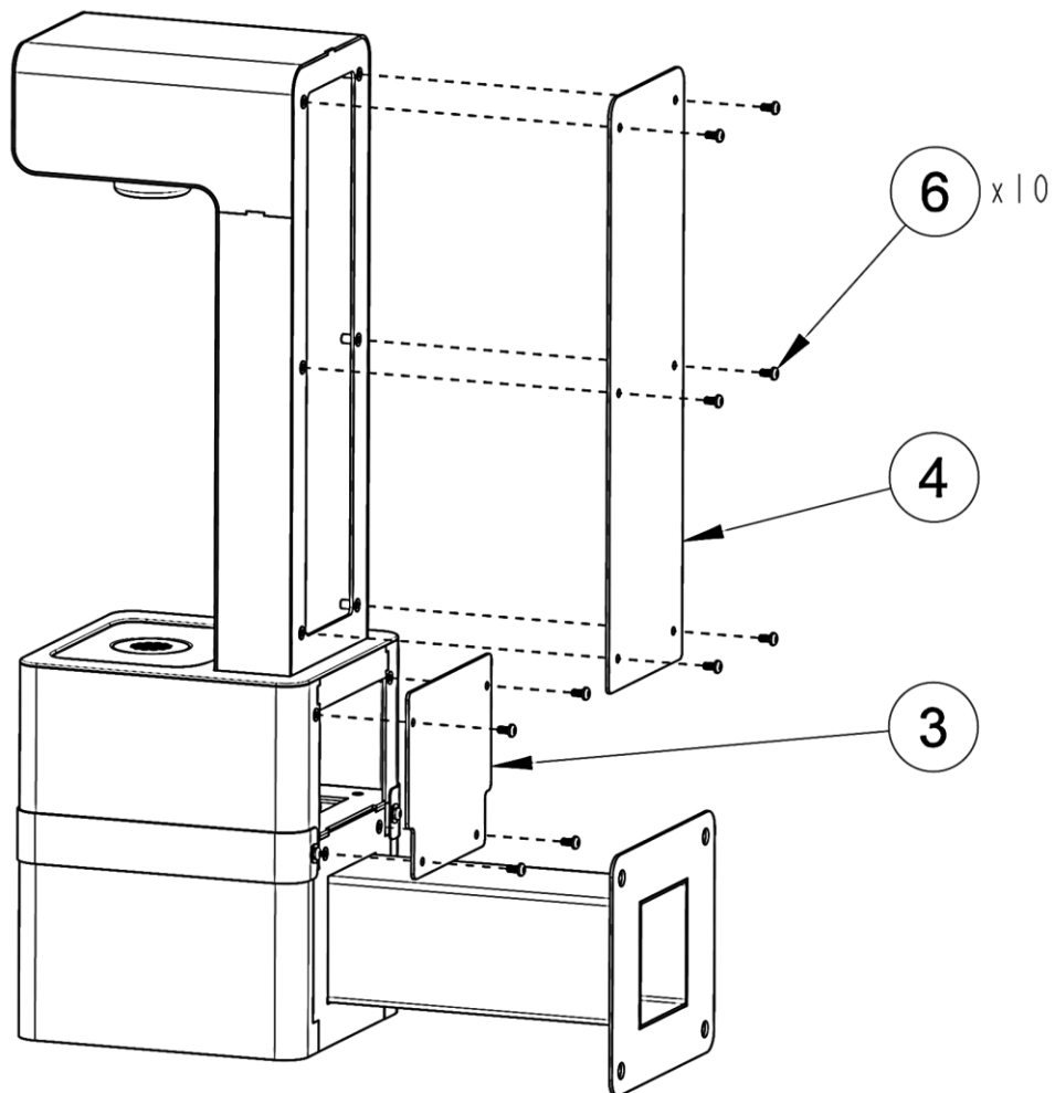
Fig.6 – Back plates assembly
