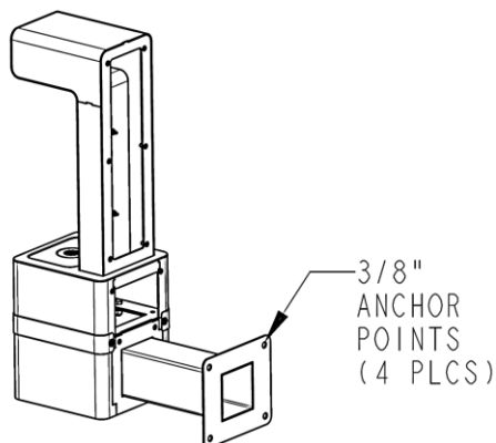
Fig.4 – Anchor points
