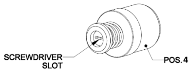
Fig. 5 – Cartridge
