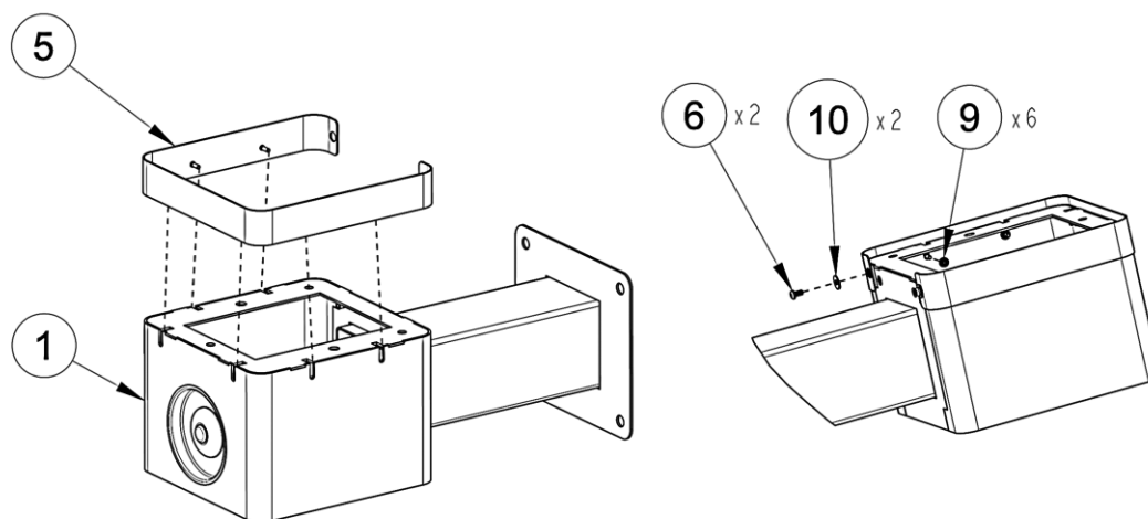
Fig. 2 – Aesthetic ring assembly
