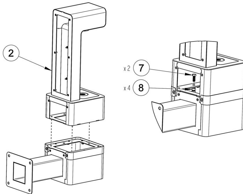
Fig.3 – Alcove assembly
