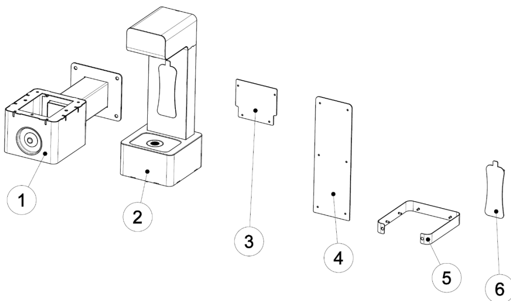
Fig. 1 – Components
