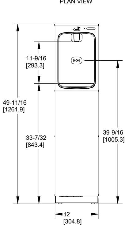
PLAN VIEW
