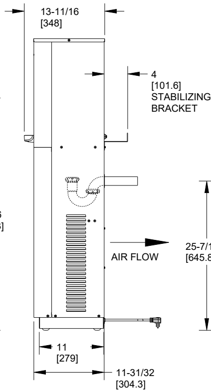
RIGHT SIDE
